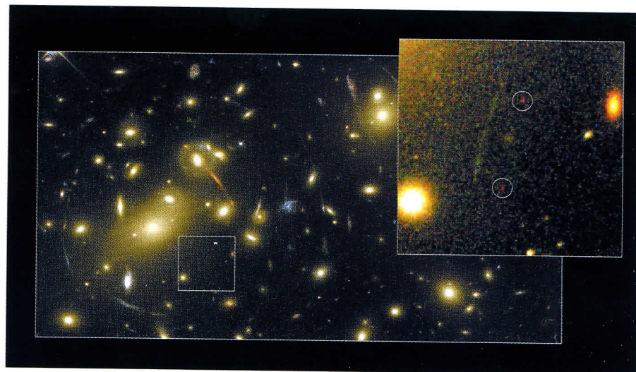
Dutch astronomers in an international team used a 'gravitational lens' to find this extremely distant 'baby'-galaxy at more than 13 billion light years. The image (insert) was magnified and split in two by the gravity of the foreground galaxy cluster Abell 2218 (courtesy NASA/HST/Kuijken).
