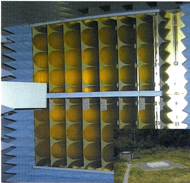
The Thousand Element Array (THEA) tile. This world first wide-band array antenna is the result of an international R&D program sponsored by NWO for the Square Kilometer Array (SKA). Insert shows the test location in Dwingeloo where 16 THEA tiles comprise a small radio telescope of a new generation (courtesy ASTRON).
