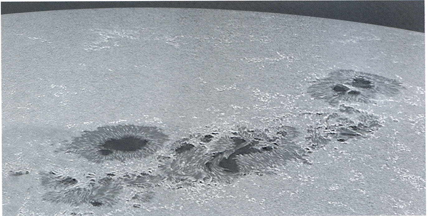
A giant group of sunspots, observed with the Dutch Open Telescope on 2 April 2001. Later on this day, the group caused the eruption of the biggest solar flare in 25 years. The picture has a resolution of 0".2 (150 km) and is a mosaic of 10 images at a wavelength of 430.5 nm (courtesy DOT).
