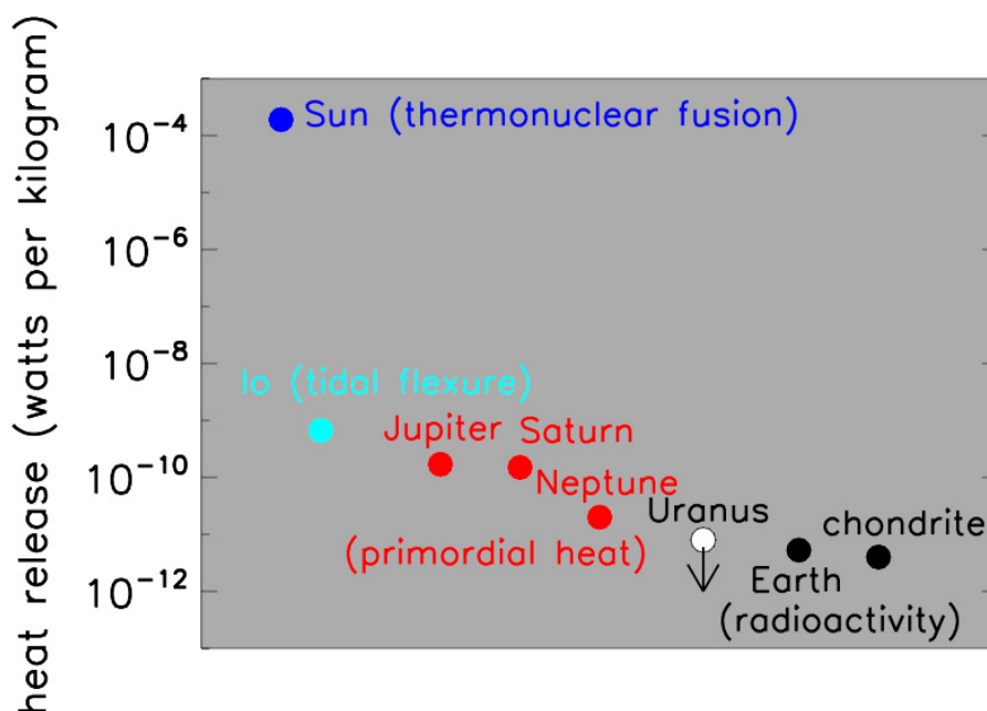
FIGURE 7.4 The intrinsic specific luminosities of some solar system objects are arrayed horizontally by predominant regimes of internal heat production at the present epoch. The Sun derives quasi-steady heating through thermonuclear fusion, while heating from tidal flexure is important in Io and possibly in some exoplanets. Jupiter, Saturn, and Neptune predominantly release primordial accretional heat. In Earth and other rocky objects of roughly chondritic composition, radioactive decay is important for heat production. SOURCE: Courtesy of William Hubbard, University of Arizona.
