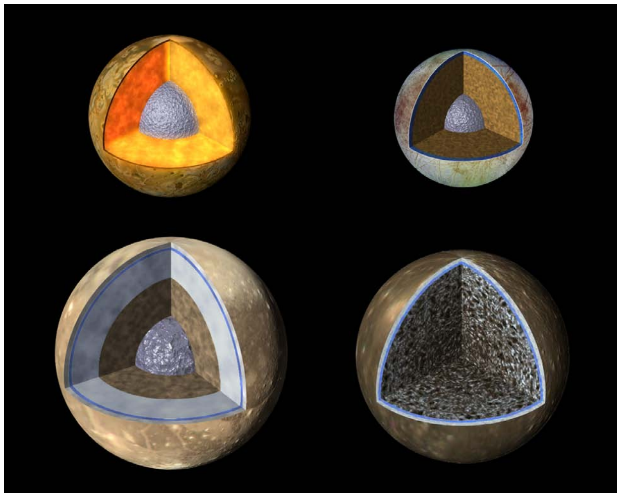
FIGURE 8.2 Schematic of the highly diverse interiors of the Galilean satellites, inferred from Galileo data. Io (upper left), Europa (upper right), and Ganymede (lower left) have metallic cores surrounded by silicate mantles which, in the case of Europa and Ganymede, are overlain by water ice and subsurface oceans (blue). Europa's ocean, unlike Ganymede's, is in contact with the underlying silicate mantle. Callisto (lower right) also hosts an ocean, but is only partially differentiated, and its interior consists primarily of mixed silicates and ice. Ganymede's diameter is 5262 km. SOURCE: NASA/JPL.
