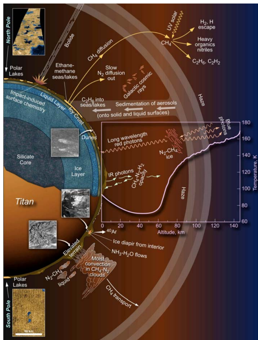
FIGURE 8.8 Schematic of the complexities of atmospheric processes on Titan, and their relationship to its surface and interior. SOURCE: NASA and ESA, Titan Saturn System Mission (TSSM) NASA/ESA Joint Summary Report , January 19, 2009. Courtesy of NASA/ESA.
