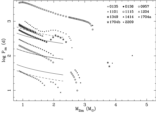
Fig. 8. Results of the spiral-in calculations, each individual symbol is a solution of the calculations and thus represents one pre-CE binary. The figure shows the logarithm of the orbital period of the intermediate binary P_m as a function of the secondary mass M_{2m} . Different symbols represent different observed systems, as explained in the legend. System 1704a is the system listed in Table 1, 1704b is the same system, but with the reverse mass ratio. For solutions with M_{2m} < 2.5 M_\odot , only every third solution is plotted for clarity. Around M_{2m} = 1.2 and \log P_m = 2.8 the symbols of WD 0135–052, WD 0136+768 and WD 1204+450 overlap due to the fact that they have similar white-dwarf masses. For comparison we show the lines of the solutions for (top to bottom) WD 0136+768, WD 0957–666 and WD 1101+364 taken from Nelemans et al. (2000), as described in the text.
