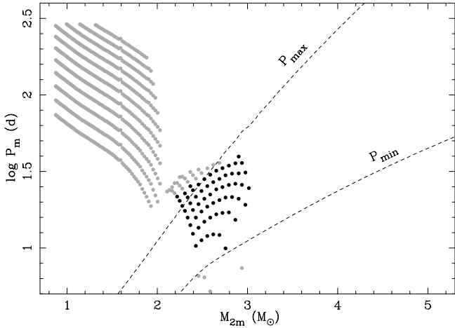
Fig. 11. Results of the spiral-in calculations for WD 0957–666 with period limits for a conservative first mass transfer. This figure contains the same data as the third panel in Fig. 10 (symbols) plus the period limits P_{\min} and P_{\max} (dashed lines). The solutions that lie between these limits are shown in black, the others in grey. See the main text for details.
