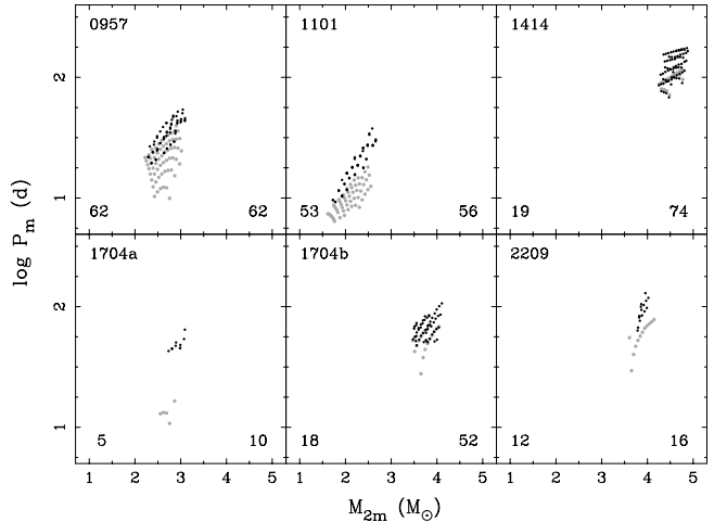
Fig. 13. Results of the spiral-in calculations (grey symbols), obtained as in Fig. 11, and the solutions of calculations of conservative evolution (black symbols). Only the six systems shown have spiral-in solutions within the period limits (see Fig. 12). The numbers in the lower left and lower right corners are the numbers of plotted spiral-in solutions and conservative solutions respectively.
