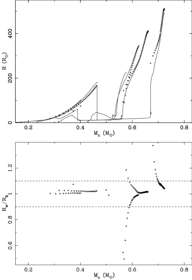
Fig. 7. Comparison of a selection of grid models with C_{\text{rml}} = 1.0 with initial masses of 1.3, 1.6, 2.0, 2.5 and 3.2 M_\odot to the basic models ( C_{\text{rml}} = 0.0 ). Upper panel a ): comparison of the radius of the models with a stellar wind (solid lines) and the radius of a basic model with the same mass and core mass (plusses). Lower panel b ): the fraction of the radius of the wind model R_w over the radius of the basic model R_b with the same total and core mass. Each data point corresponds to a point in the upper panel. Of the data points in the upper panel, 7 out of 143 (5%) lie outside the plot boundaries in the lower panel. The dashed horizontal lines show the region where agreement is better than 10%, where 83% of the data points lie. The 1.0 M_\odot model was left out because there are only a few basic models with lower mass, the higher-mass models were left out because they lose very little mass (see Fig. 5).
