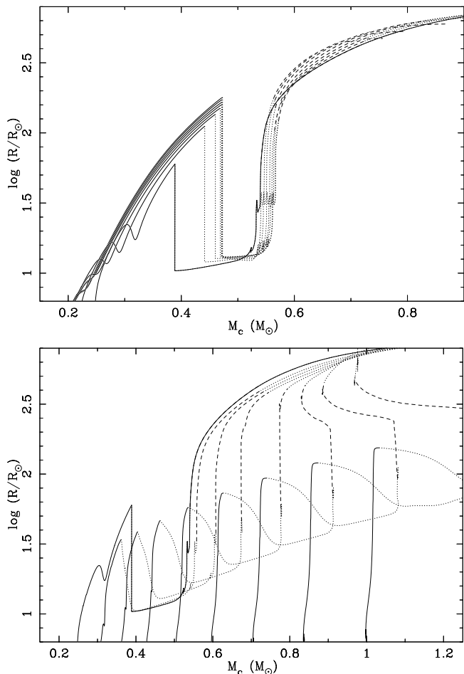
Fig. 1. Core-mass – radius relations for the “basic” models, as described in the text. The lines show the logarithm of the radius of the stars as a function of the helium-core mass. Upper panel a ): low-mass grid models with masses of 0.91, 1.01, 1.14, 1.30, 1.48, 1.63, 1.81 and 2.00 M_{\odot} . Lower panel b ): high-mass grid models with masses of 2.00, 2.46, 2.79, 3.17, 3.60, 4.09, 4.65, 5.28 and 6.00 M_{\odot} . The 2 M_{\odot} model is plotted in both panels throughout as a solid line for easier comparison. The other models are shown as solid lines on the first giant branch (FGB), where they could cause a common envelope resulting in a spiral-in and creating a helium white dwarf. The dashed lines show the asymptotic giant branch (AGB), where a common envelope would lead to the formation of a carbon-oxygen white dwarf. Dotted lines are parts of the evolution where the stars either are smaller than at the tip of the FGB (at lower radii) or where their envelope binding energies become positive on the AGB (at large radii).
