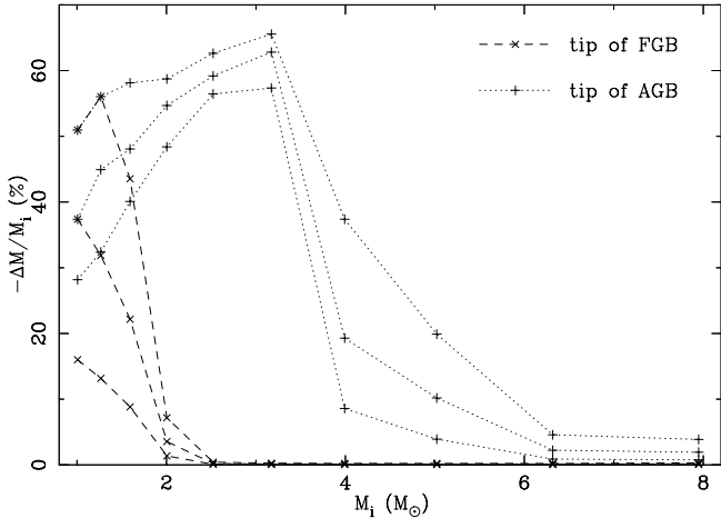
Fig. 5. The fraction of mass lost at two moments in the evolution of a star as a function of its initial mass, for the three different wind strengths ( C_{\text{rml}} = 0.2, 0.5 and 1.0 ) used in the grid. This fraction is shown for the tip of the FGB (dashed lines and crosses), and the “tip of the AGB” (dotted lines and pluses). See the text for details.
