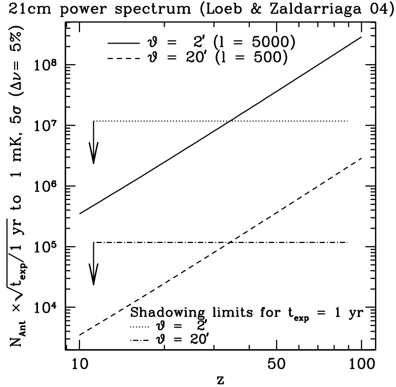
Fig. 13. Number of antennas necessary to achieve a 5\text{-}\sigma detection of fluctuations in the 21 cm power spectrum in one year at multipole numbers up to l = 5000 (corresponding to 2' angular resolution) or l = 500 ( 20' ) at the 1 mK level, as function of redshift (as given by eq. 11 from Loeb and Zaldarriaga, 2004). Except for the different exposure time prescription, this figure is constructed in the same way as Fig. 11, so that the same scalings apply, i.e. , N_{\text{Ant}} \sqrt{t_{\text{exp}}} S^{-1} l^{-2} (1+z)^3 = \text{const} (where S is the desired sensitivity level), assuming a filling factor independent of frequency.
