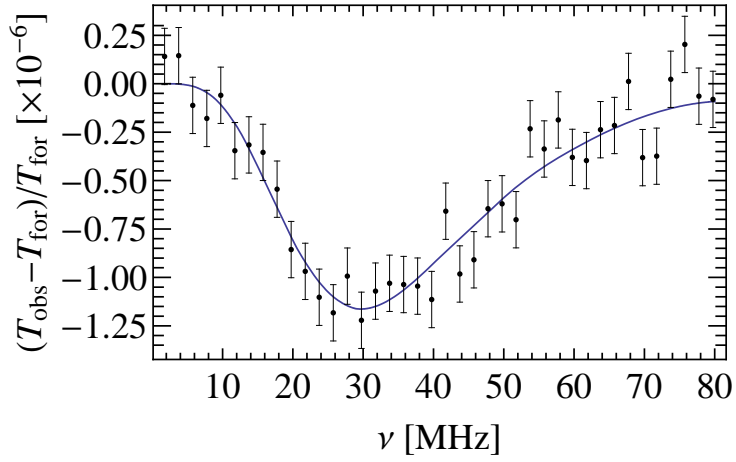
Fig. 9. A simulated global 21-cm HI signal from the dark ages after 1 year of integration time with a single sky-noise limited dipole as a function of frequency (based on the calculations by Ciardi and Salvaterra, 2007, also compare Fig. 10). Here a fixed bandwidth of 1.5 MHz is used. We assume that the observed brightness temperature, T_{\text{obs}} , is just the sum of the dark ages signal and a foreground signal, T_{\text{for}} , which is a perfect power law. The signal at 30 MHz originates from z = 46 .
