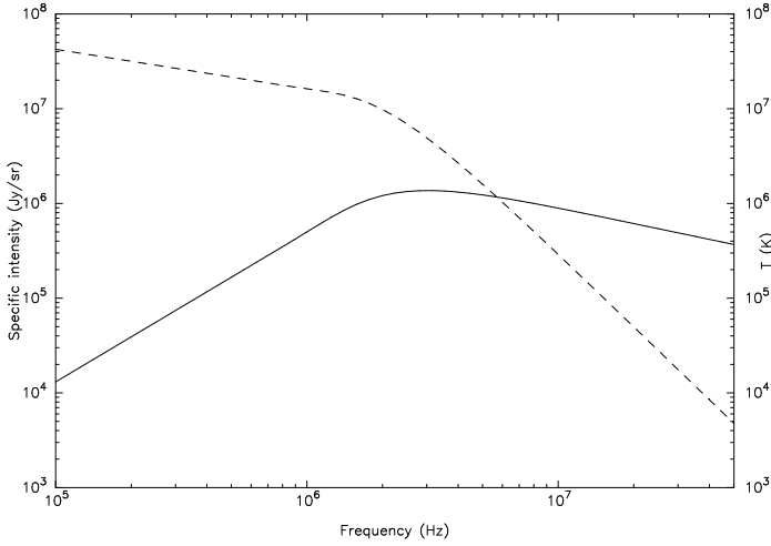
Fig. 3. Spectrum of Galactic synchrotron emission, showing specific intensity (solid line) and surface brightness temperature (dashed line). The surface brightness temperature dominates the system temperature at the frequencies shown. Figure taken from Oberoi and Pinçon (2003).
