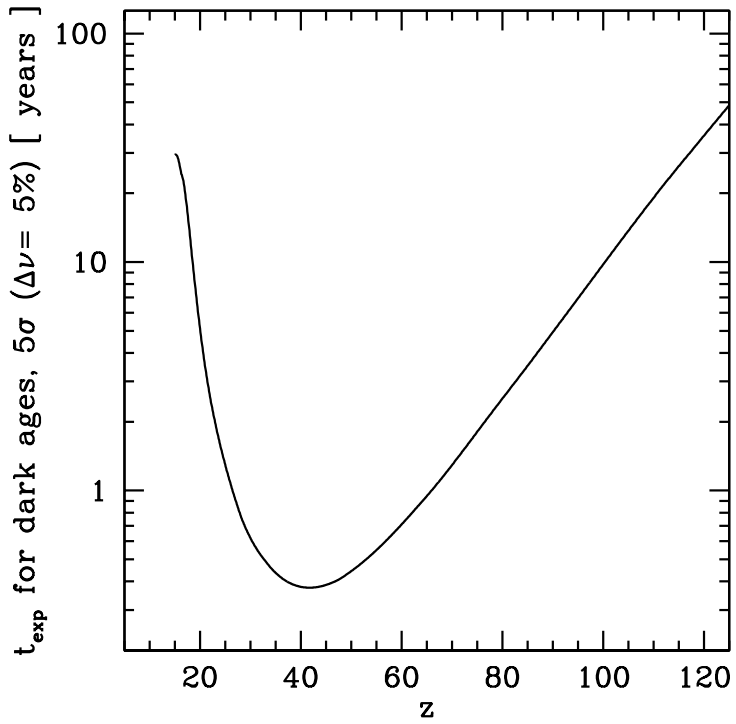
Fig. 10. Global 21-cm signal from HI in the dark ages. The plot shows the observing time needed to reach a 5\text{-}\sigma detection at 5% fractional bandwidth with a single dipole, as function of redshift. If N dipoles are added incoherently, then the observing time is reduced by a factor \sqrt{N} .
