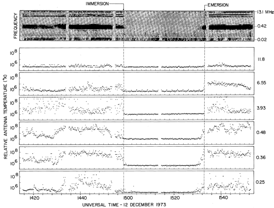
Fig. 1. Shielding of terrestrial radio interference by the moon, as observed by the RAE-2 satellite. Even at a distance of 300,000 km from the Earth, the additional shielding by the Moon provides 1-3 orders of magnitude (10-30 dB) of additional interference suppression. Taken from Alexander et al. (1975, © ESO).
