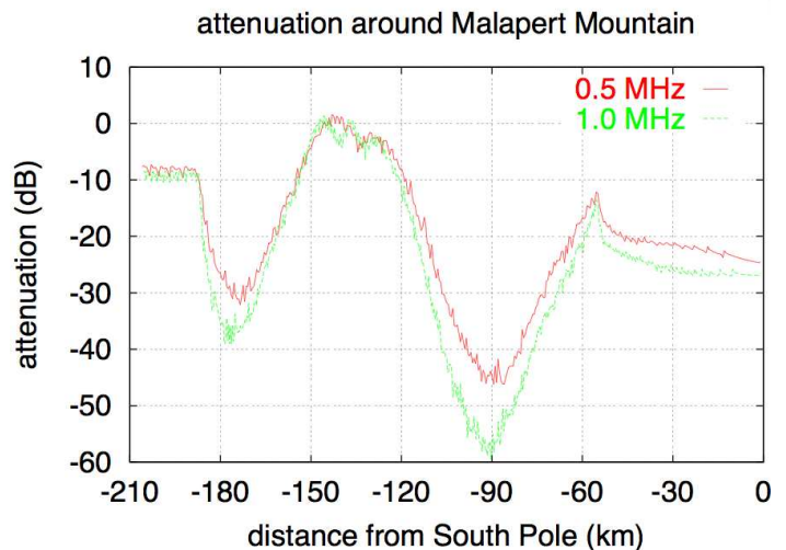
Fig. 2. Shielding of terrestrial radio interference by Malapert mountain, whose peak is at \approx 120 km from the south pole. This shielding is in addition to the 20–30 dB attenuation applying to all interference in the south polar region. Taken from Takahashi (2003, Fig. 4.9) with kind permission of the author.
