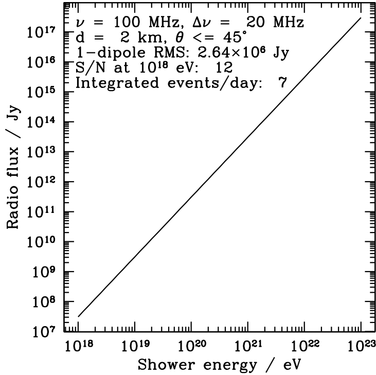
Fig. 16. Radio flux from cosmic-ray or neutrino events interacting with the Moon, as observed at 100 MHz with a single dipole located on the Moon. The flux and event rate were computed using the formulae given by Scholten et al. (2006).
