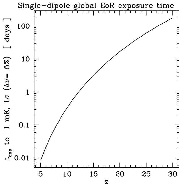
Fig. 8. Integration time necessary to reach an RMS noise level of 1 mK in the redshifted 21-cm line for observing the global Epoch of Reionization signal (of order of a few to a few tens of mK; Gnedin and Shaver, 2004, Fig. 1) with a single dipole against the Galactic foreground emission, as function of redshift ( z = 5 corresponds to \nu = 230 MHz, z = 30 to 45 MHz) The integration time is obtained from eqns. 5 and 7 with f = 1 . A constant fractional bandwidth of 5% was assumed. To reach fainter noise levels s , the required integration time scales as t_{\text{exp}} \propto 1/s^2 . The redshift range shown includes the entire likely range for the origin of the global EoR signal; redshifted 21-cm emission from higher redshifts is considered separately below.
