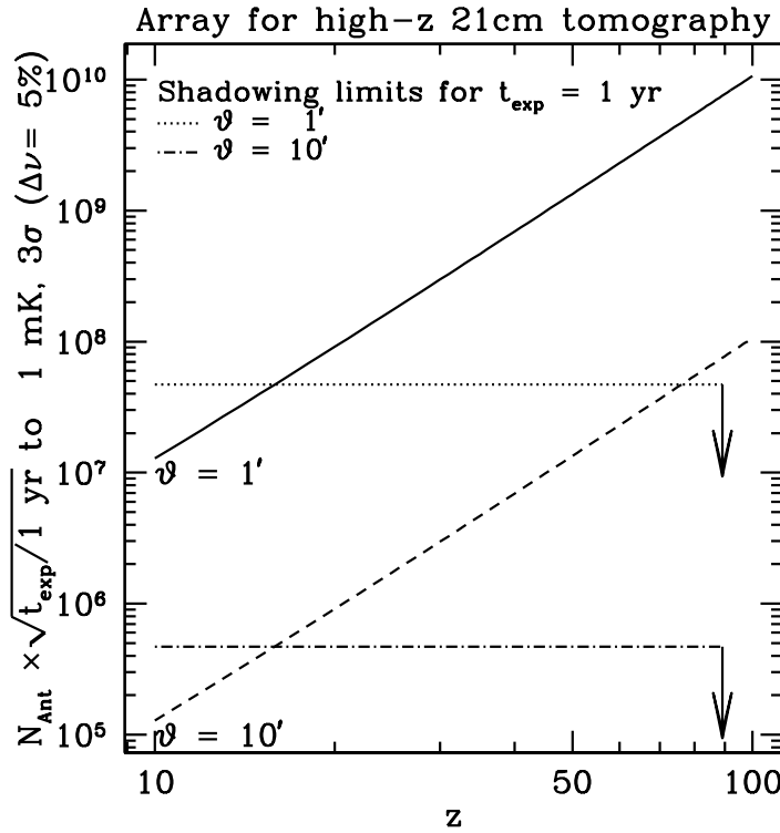
Fig. 11. Number of crossed dipoles (from eq. [4]) required for a 3\text{-}\sigma detection of 1 mK per resolution element in one year when imaging the redshifted 21cm emission at frequency \nu_{21}(z) = 1.4\text{ GHz}/(1+z) at angular resolution \theta = 1' , assuming a constant filling factor independent of wavelength (i.e., a scaled array). The required number of crossed dipoles to achieve this RMS can be traded against longer exposure times (and vice versa ) as indicated, but must not exceed the shadowing limit from eq. (9), N < N_{\text{max}} = 4.7 \times 10^7 (\theta/1')^{-2} . The corresponding collecting area is given by 1.1 \times 10^{-8} N(1+z)^2 \text{ km}^2 . The array diameter (or maximum baseline) required to reach a given resolution is shown in Fig.5 and ranges from \approx 800\text{m} ( z = 10, \theta = 10' ) to \approx 80\text{m} ( z = 100, \theta = 1' ). The numbers from this graph can be scaled as N_{\text{Ant}} \sqrt{t_{\text{exp}}} S^{-1} \theta^2 (1+z)^3 = \text{const} (where S is the desired sensitivity).
