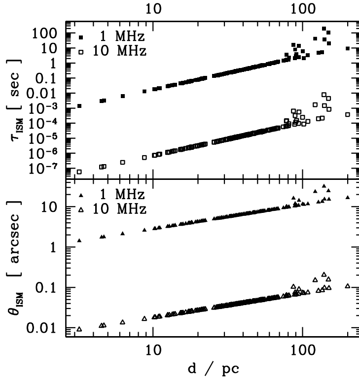
Fig. 15. Pulse broadening times (top panel) and angular broadening scales (bottom panel) caused by ISM turbulence towards known extrasolar planets, as calculated from the NE2001 model for the distribution of free electrons in the Galaxy (Cordes and Lazio, 2002). The temporal and angular broadening is shown for the two different frequencies as indicated; the strength of the former scales as \nu^{-4.4} , that of the latter as \nu^{-2.2} . The angular broadening is always negligible compared to the likely resolution of a lunar array (compare Fig. 5). The temporal broadening at 1 MHz is short compared to the likely exoplanetary radio burst duration of \approx 15 minutes for all but the most distant planets behind those ISM regions with the strongest turbulence.
