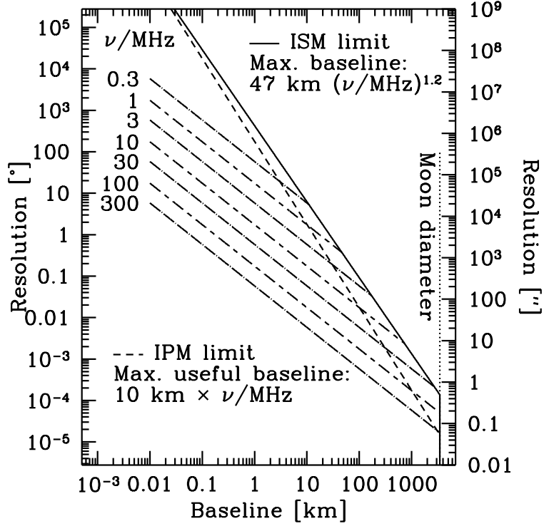
Fig. 5. Resolution of a radio array as function of baseline. The ISM and IPM scattering limits are also shown, assuming the scattering laws given by Woan (2000). The ISM scattering size is in principle a firm limit to the resolution achievable for extragalactic observations, but could be smaller in some small part of the sky, in particular away from both the Galactic plane and the Galactic centre. The IPM scattering has not been measured well at low frequencies and could be a factor 15 smaller than given. The IPM scattering is given here for the anti-solar direction; it will increase when observing closer to the sun, and vary with the solar cycle.
