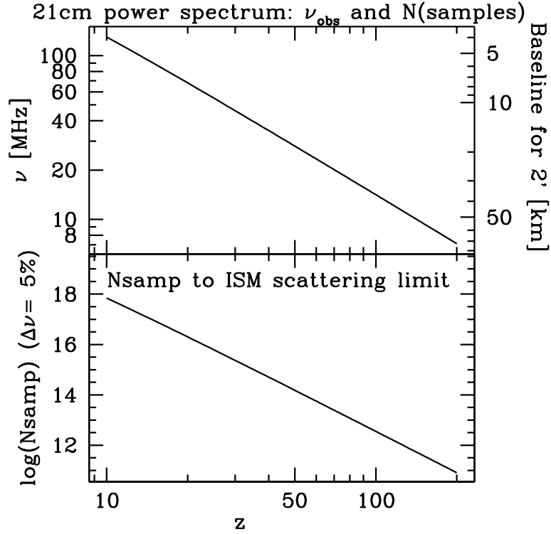
Fig. 12. Upper panel: observed frequency of redshifted 21cm emission (left-hand axis), and baseline required to reach 2' resolution at that frequency (right-hand axis), both as function of redshift z . Ground-based observations are exceedingly difficult below 30 MHz, corresponding to z = 47 . Lower panel: Number of independent power-spectrum samples ( N_{21\text{cm}} from Loeb and Zaldarriaga, 2004, p. 4) obtainable down to the ISM scattering limit towards the Galactic poles, also as function of redshift.
