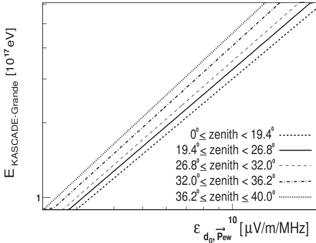
Figure 6: Linear fits for the energy – radio amplitude in d_0 correlation (double-log scale), for all the zenith angle bins. The slope of each fit clearly depends on the inclination of the air shower.
