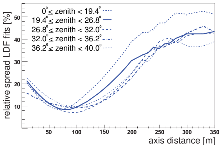
Figure 4: Relative RMS-spread profile for the CoREAS LDF fits as a function of distance from the shower axis, for the different zenith angle bins.
