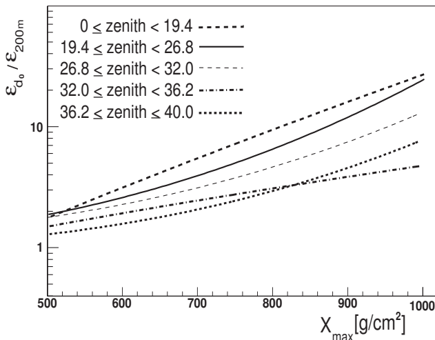
Figure 9: Fits as in fig. 8 but for each zenith angle bin. The expected dependence of the X_{\max} -radio LDF slope correlation on the zenith angle is clearly visible.
