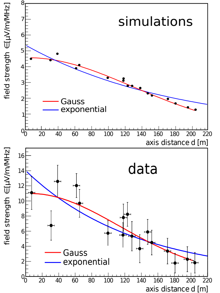
Figure 2: Lateral distribution functions for an event in the selection used for the analysis. A Gaussian and an exponential function are used to fit the points. Top: CoREAS simulations. Bottom: LOPES data. The absolute amplitudes exhibit a known scale mismatch between LOPES data and CoREAS simulations (see text and ref. [10]).
