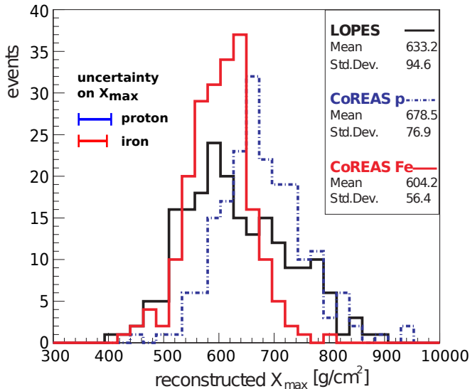
Figure 11: X_{\max} distribution reconstructed with the slope method for the LOPES measurements (black) and for the CoREAS proton (dashed-blue) and iron (light-red) simulations of the same events, for the complete zenith angle range of 0 - 40^\circ . The indicated uncertainty on X_{\max} is derived from fig. 10.
