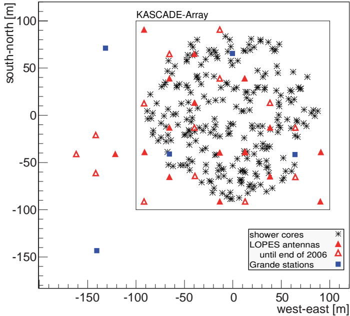
Figure 1: Shower core positions of the 205 selected events, measured simultaneously by the particle detector KASCADE-Grande and by the LOPES east-west-aligned antennas.
