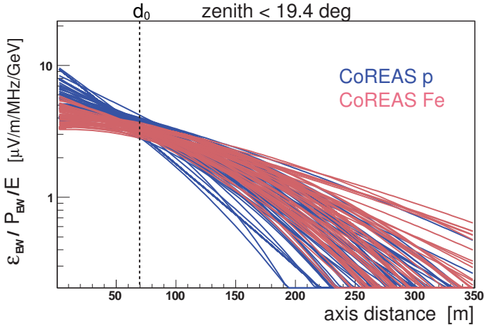
Figure 3: Normalized CoREAS lateral distribution function fits using a one-dimensional Gaussian for the events with zenith angles smaller than 19.4^\circ , simulated once as proton (blue), once as iron (light-red) primaries. The dotted line represents the distance d_0 at which the RMS-spread of the fitted normalized radio amplitudes is minimal.
