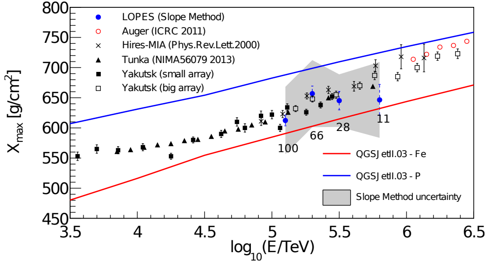
Figure 13: Mean X_{\max} as a function of the primary cosmic ray energy. The blue points correspond to the LOPES-reconstructed values, using the slope method. The errors are calculated as (\text{standard deviation}/\sqrt{\text{events}}) , and the numbers indicate our statistics in each energy bin. The lines refer to the Monte Carlo expectations for pure iron (red) and pure proton (blue) composition, using the QGSJetII-03 hadronic interaction model. Results from other experiments are indicated by markers (please see legend).
