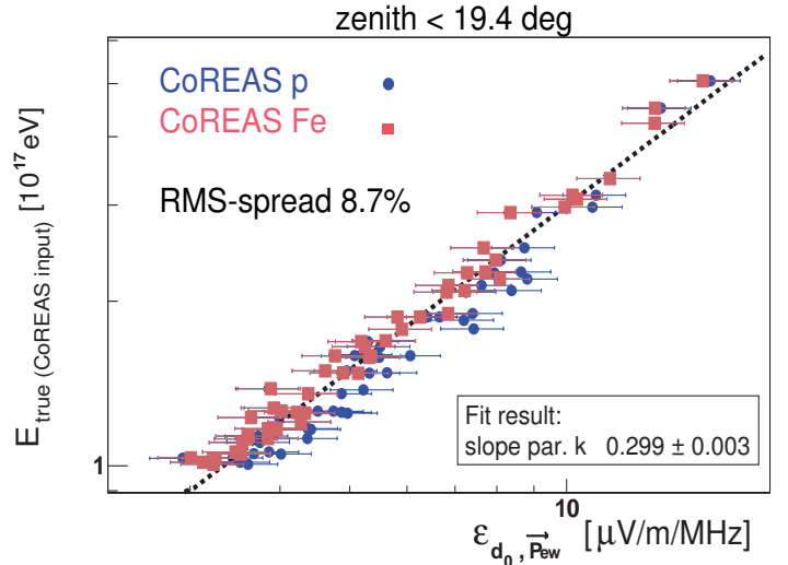
Figure 5: Linear correlation between the Monte Carlo true primary energy and the CoREAS radio pulse amplitude at the distance d_0 , with k the free parameter of the fit. The radio amplitude is normalized by the east-west component of the Lorentz force vector. The RMS-spread is \sim 8.7\% .
