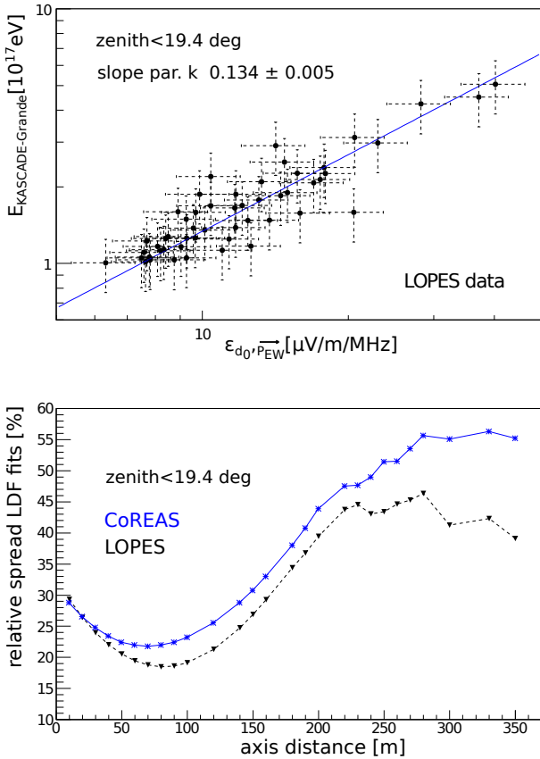
Figure 7: Top: Linear correlation of the KASCADE(-Grande) reconstructed primary energy and the normalized LOPES measured radio pulse in d_0 , for zenith angles less than 19.4^\circ . The RMS-spread is 18.8\% . Bottom: RMS-spread from the energy-fit for zenith angle less than 19.4^\circ , computed at several distances from the shower axis. With the LOPES measurements (black triangles) the minimum is found at 80 m. The blue stars represent the CoREAS predictions (fig. 4 for the same events, adding 20% for the KASCADE energy uncertainty).
