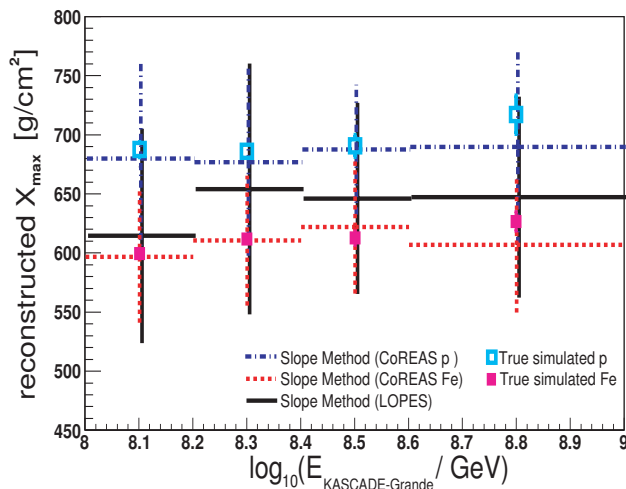
Figure 12: The energy dependence of the reconstructed LOPES X_{\max} distribution (black), compared with the CoREAS values for proton (blue-dashed line) and iron (red-dotted line) primaries, and with the Monte Carlo values for proton (light-blue marker) and iron (light-red marker) primaries.
