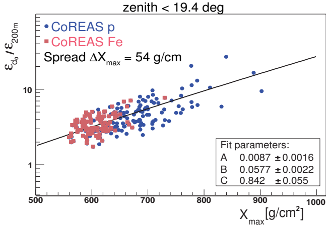
Figure 8: Correlation between the true X_{\max} from Monte Carlo simulations and the LDF slope of the CoREAS simulated radio amplitudes. The RMS-spread around the fit is \sim 54 \text{ g/cm}^2 .
