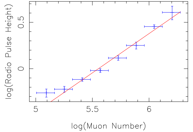
FIG. 9: Variation of the radio pulse height with the muon size of the shower after the signal amplitude has been corrected for the geomagnetic angle and the distance to the shower core [9]. The experimental point in the first bin is biased by the efficiency for a poor signal-to-noise ratio at low shower sizes.
