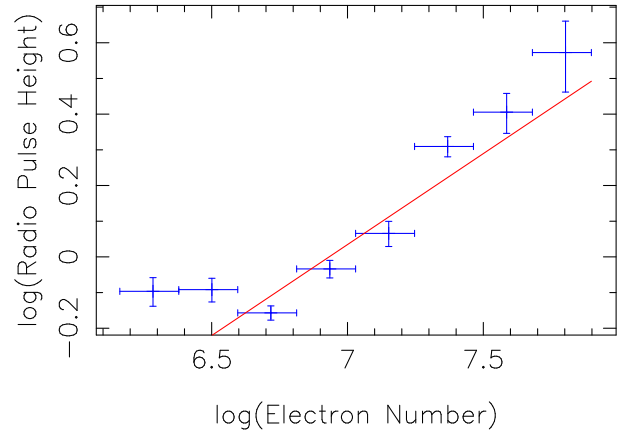
FIG. 10: Variation of the radio pulse height with the electron size of the shower after the signal amplitude has been corrected for the geomagnetic angle and the distance to the shower core [9].
