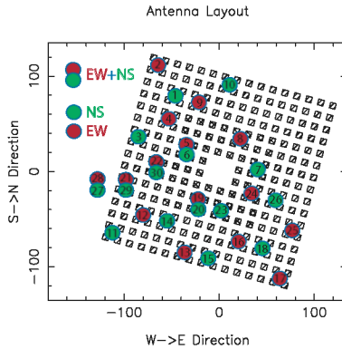
FIGURE 2. The antenna layout at the KASCADE array. The all antenna setup is divided in 15 E-W and 15 N-S polarized channels. Five antennas are sensitive to both polarization directions at the same station.
