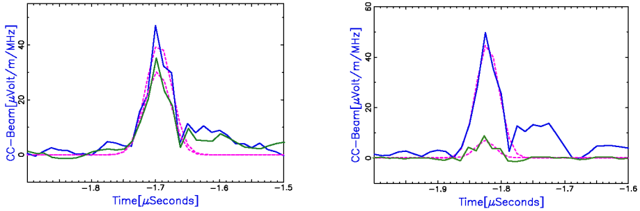
FIGURE 4. Left panel: The Cross Correlation(CC)-beams for a dual-polarized event (E-W component: upper signal, N-S component: lower signal) of a primary energy of 10^{18} eV coming from North-East. The full lines indicate the CC-beams and the dotted lines the Gaussian fits respectively. One can clearly see very high radio signal recorded in both polarization directions. Right panel: The same Cross Correlation(CC)-beam for a dual-polarized event of a primary energy of 3 \cdot 10^{17} eV coming from North, North-West. One can clearly see very high signal recorded in the E-W polarization direction only.
