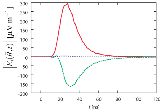
FIGURE 1. Raw simulated pulses in the individual linear polarization components of a 10^{17} eV vertical air shower. The solid line represents the E-W polarization component, dashed line N-S and dotted line the vertical component respectively.
