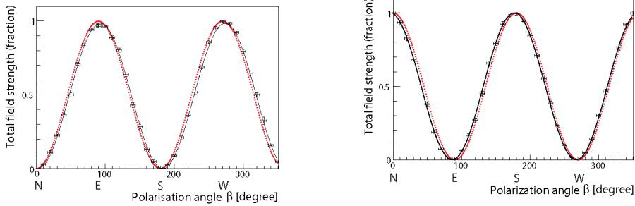
FIGURE 3. Left panel: Fraction of the total field strength seen by the linearly polarized LOPES antenna (sensitive to E-W) as a function of the polarization angle \beta . Points: experimental data, solid line: data fit by a \sin\beta -function, dotted line: theoretical \sin\beta -distribution (normalized to the value at \beta=270^\circ ). Right panel: An antenna sensitive to the N-S polarization direction of the radio signal. The dotted curve is normalized to the value at \beta=180^\circ .
