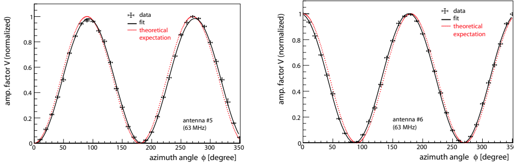
(a) Polarization measurements at 63 MHz for antenna #5, amplification factor normalized to the maximum at \phi = 270^\circ
