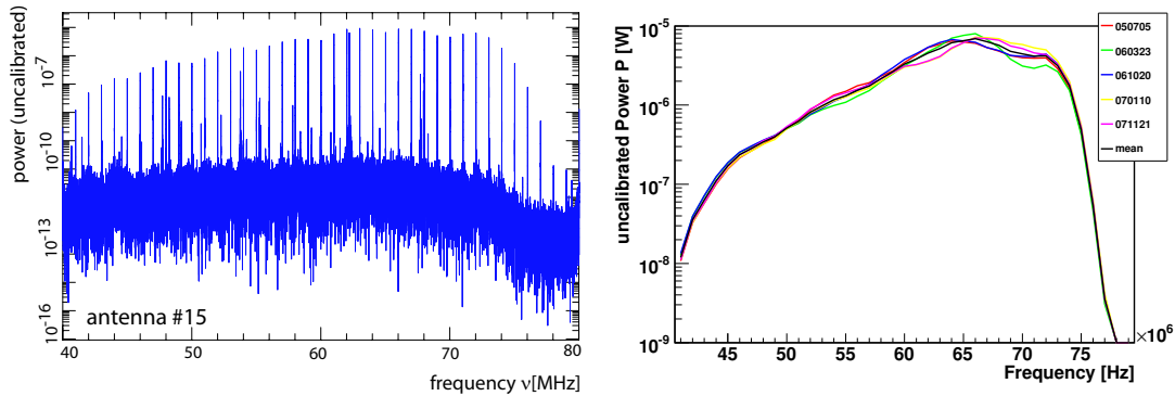
(a) Measured power of one calibration raw data file. Clearly visible are the 1 MHz steps of the emission of the reference antenna with its comb generator.
