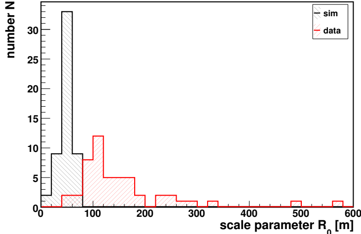
Figure 5.21: Distribution of the scale parameter R_0 obtained from measurements (red histogram) and simulations (black histogram).
