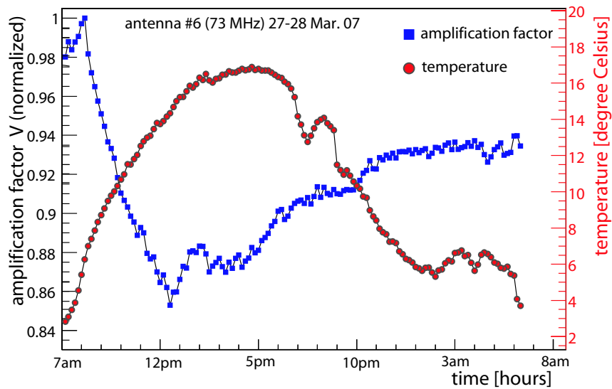
(a) Relation of amplification factor V (73 MHz), normalized to the highest values, over time and the diurnal cycles of the air temperature at 2 m height over time.
