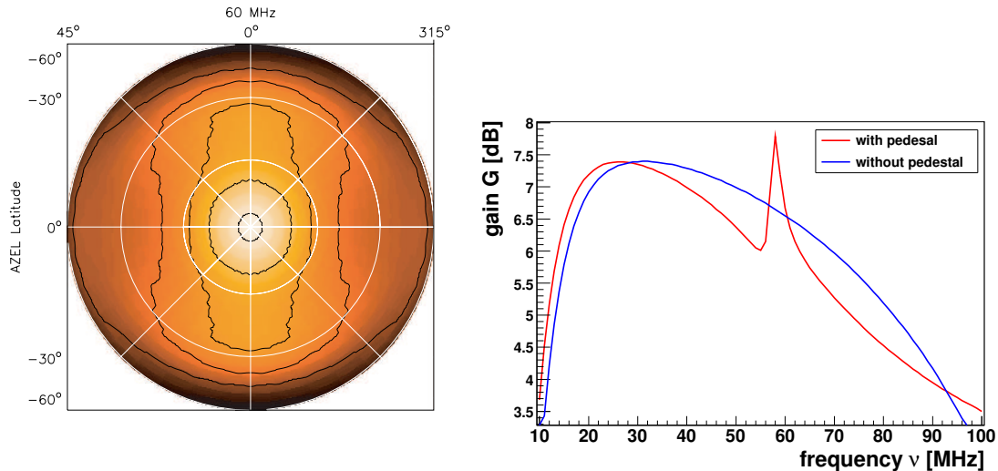
Figure 3.3: Left: Modeled antenna gain patterns for the LOPES antenna at 60 MHz. The polar plot shows the zenith in the center and the horizon at the plot edges, with a horizontally oriented antenna. The gain is color-coded and ranges from black (minimum) to the white (maximum). Dark contours are plotted in steps of 20% of the gain. Right: Comparison of the gain in the zenith for a LOPES antenna with (red line) and without (blue line) a pedestal. For the antenna calculation with pedestal a sharp resonance is obtained at 58 MHz.
