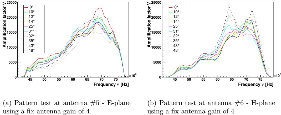
Figure 4.15: Amplification factors obtained using a fixed antenna gain. Left: antenna #5 sensitive to the E-plane. Right: antenna #6 sensitive to the H-plane.
