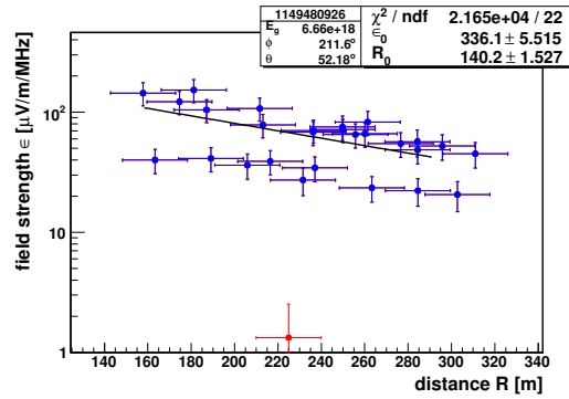
(d) Very unusual distribution with seemingly two groups of lateral distributions.
