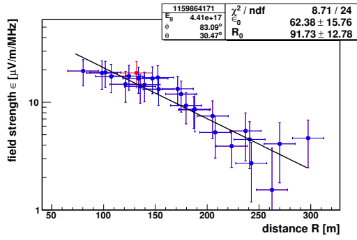
(a) Slope change at about 140 m. Flattening of the lateral shape closer to the shower center.
