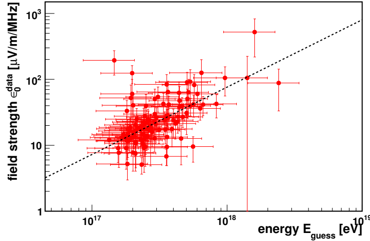
Figure 5.17: The field strength at the shower center \epsilon_0 as a function of the primary energy E_{\text{guess}} . \epsilon_0 is the result of a fit to the lateral distribution of single events. The diagonal is following a power law with index \kappa = 1 .
