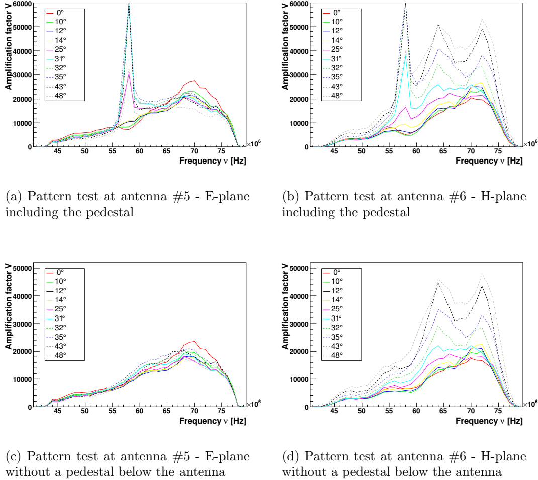
Figure 4.14: Comparison of amplification factors for two antennas, equipped as dual polarized antenna, amplification factors for different zenith angles are shown. The calculations include the pedestal (upper row) or use an antenna placed at the ground (lower row). The E-plane (left column) and the H-plane (right column) could be tested with this measurement for different zenith angles up to 48^\circ .
