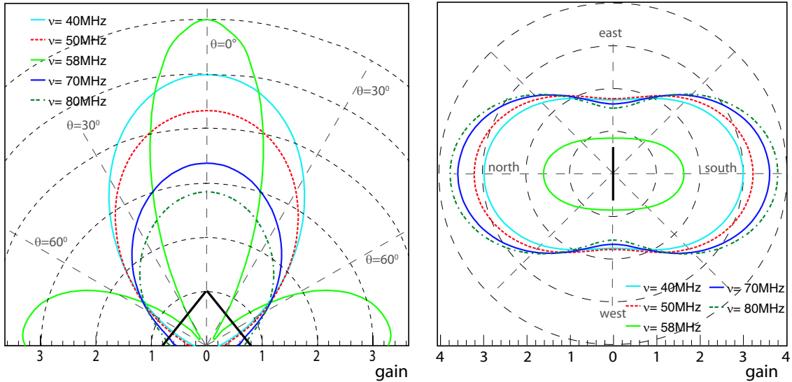
Figure 3.2: Left: Antenna gain G_r(\theta, 180^\circ, \nu) of the LOPES antenna in the \vec{E} -plane (zenithal sensitivity). The antenna is illustrated by a triangle in the center of the x-axis and lies in the image plane. Right: Antenna gain G_r(45^\circ, \phi, \nu) of the LOPES antenna for a fixed zenith angle (azimuthal sensitivity). This can be considered as a horizontal plane cut at \theta = 45^\circ . The dipole antenna lies on the y-axis.
