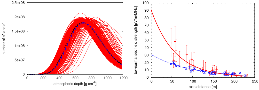
Figure 5.20: Left: 250 showers simulated with CONEX (red lines) and one representative (black line), that was used for a CORSIKA simulation (blue line). Right: Lateral distribution shown for R_0 from data and simulations.
