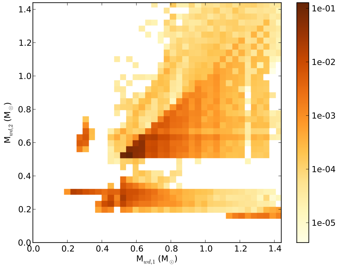
Binary_c
